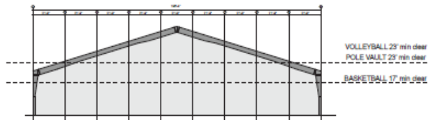
BUILDING SECTION | height clearances
